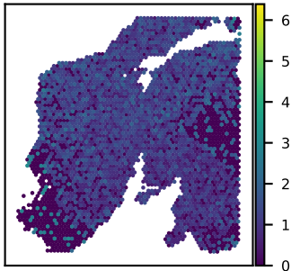
SNU24A SPATA20 expression Moran's I = 0.16
