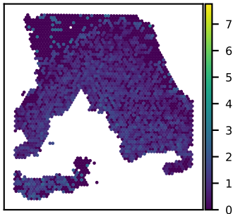
SNU18A PTPRF expression Moran's I = 0.20
