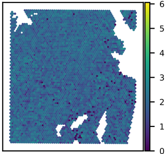
SNU51A NRCAM expression Moran's I = 0.06
