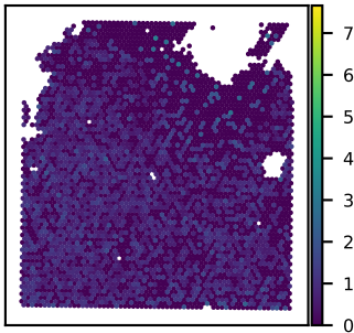
SNU21B CLCN6 expression Moran's I = 0.07
