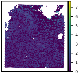
SNU21B HIST1H2AE expression Moran's I = 0.08
