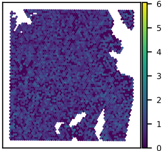
SNU51A DMAP1 expression Moran's I = 0.03
