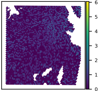
SNU51A FBXW7 expression Moran's I = 0.08
