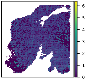
SNU24A C11orf49 expression Moran's I = 0.11
