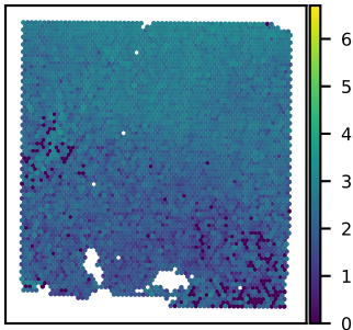
SNU43A FCGRT expression Moran's I = 0.50
