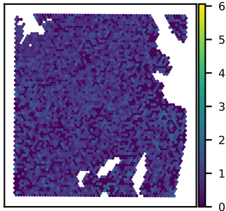
SNU51A LEPROT expression Moran's I = 0.03
