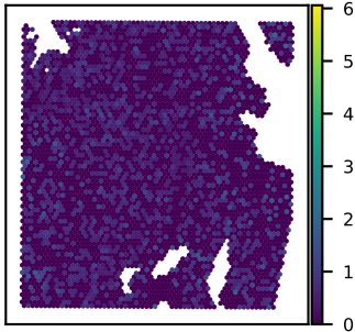
SNU51A TRAPPC9 expression Moran's I = 0.01
