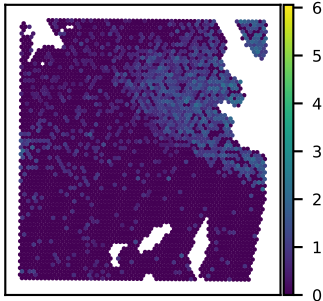
SNU51A FRRS1L expression Moran's I = 0.46
