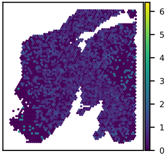
SNU24A AGO3 expression Moran's I = 0.05
