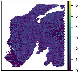
SNU24A HIBADH expression Moran's I = 0.05
