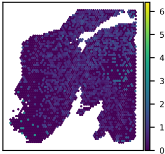
SNU24A SMPDL3A expression Moran's I = 0.10
