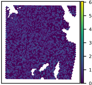
SNU51A ZNF226 expression Moran's I = 0.01
