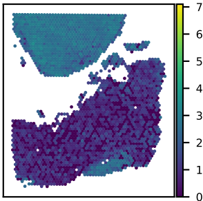
SNU25A TMEM59L expression Moran's I = 0.75
