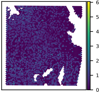
SNU51A ANGPTL2 expression Moran's I = 0.09
