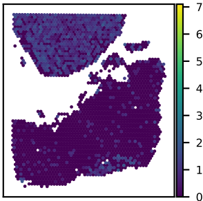
SNU25A UNC5A expression Moran's I = 0.44
