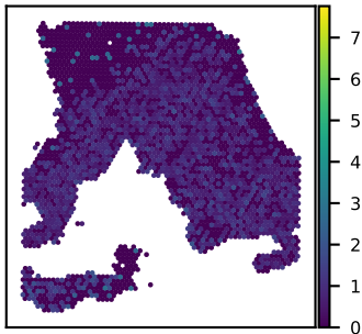
SNU18A SACM1L expression Moran's I = 0.08
