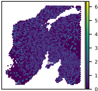
SNU24A NUDT2 expression Moran's I = 0.08
