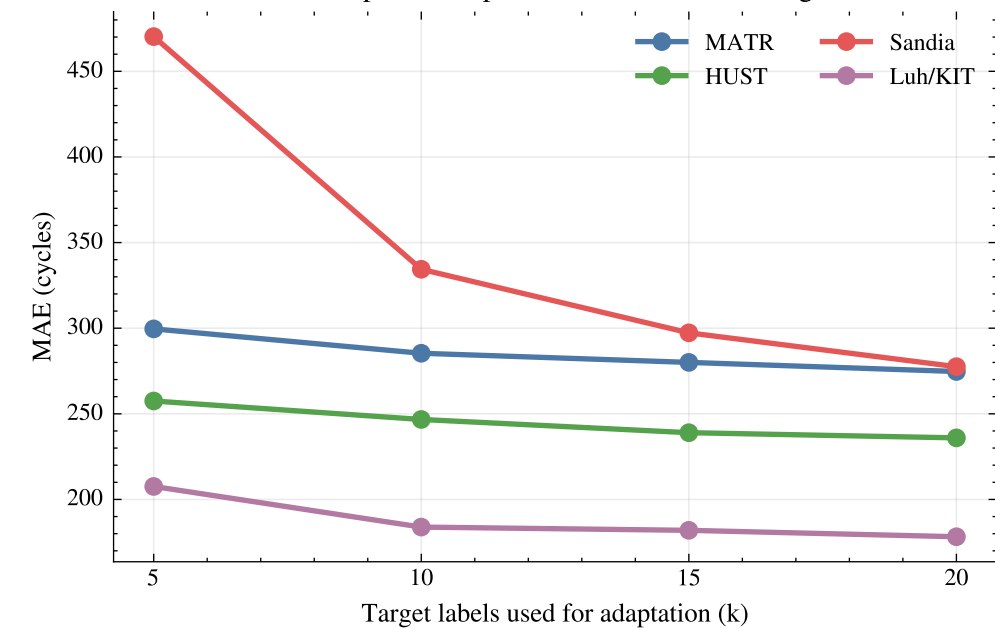
C. LODO adaptation improves MAE with more target labels
