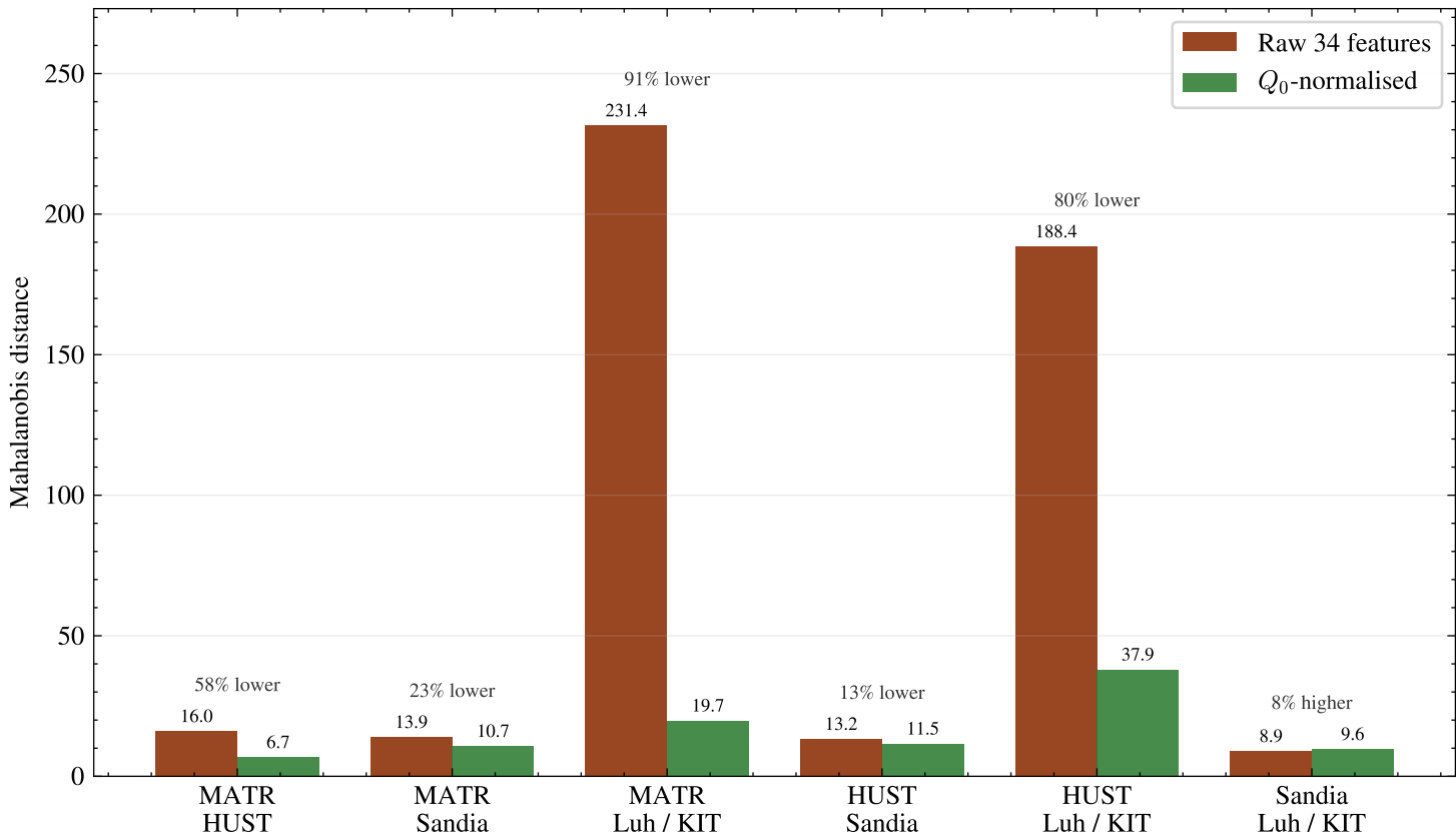
Mahalanobis distance: raw vs Q_0 -normalised features
