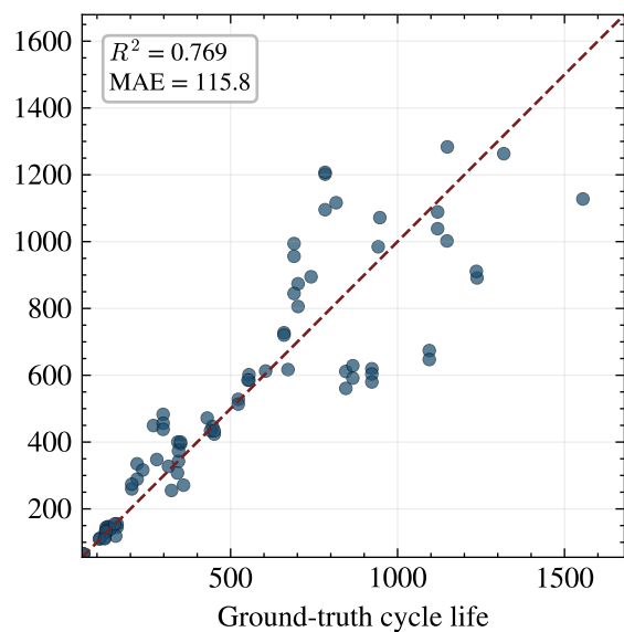
Luh / KIT - Gaussian Process
