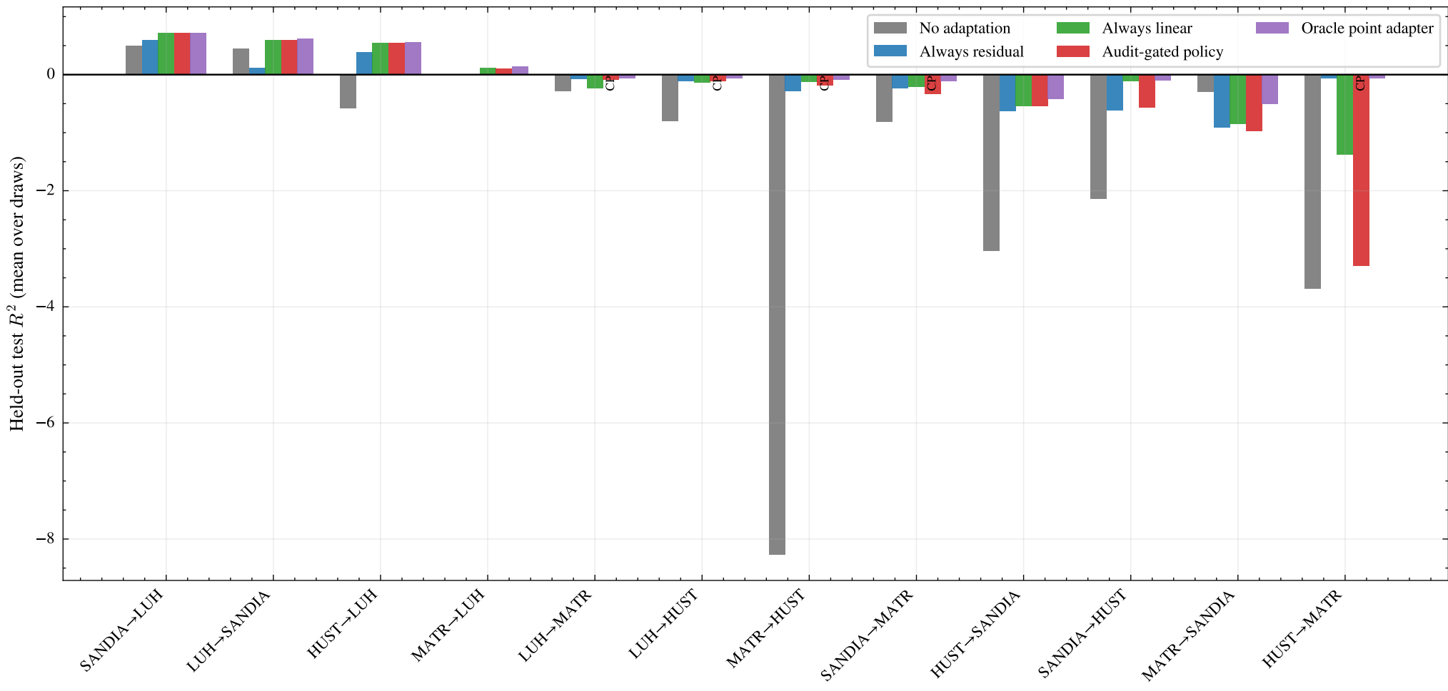
Prospective k=20 audit-gated policy vs fixed adapters
