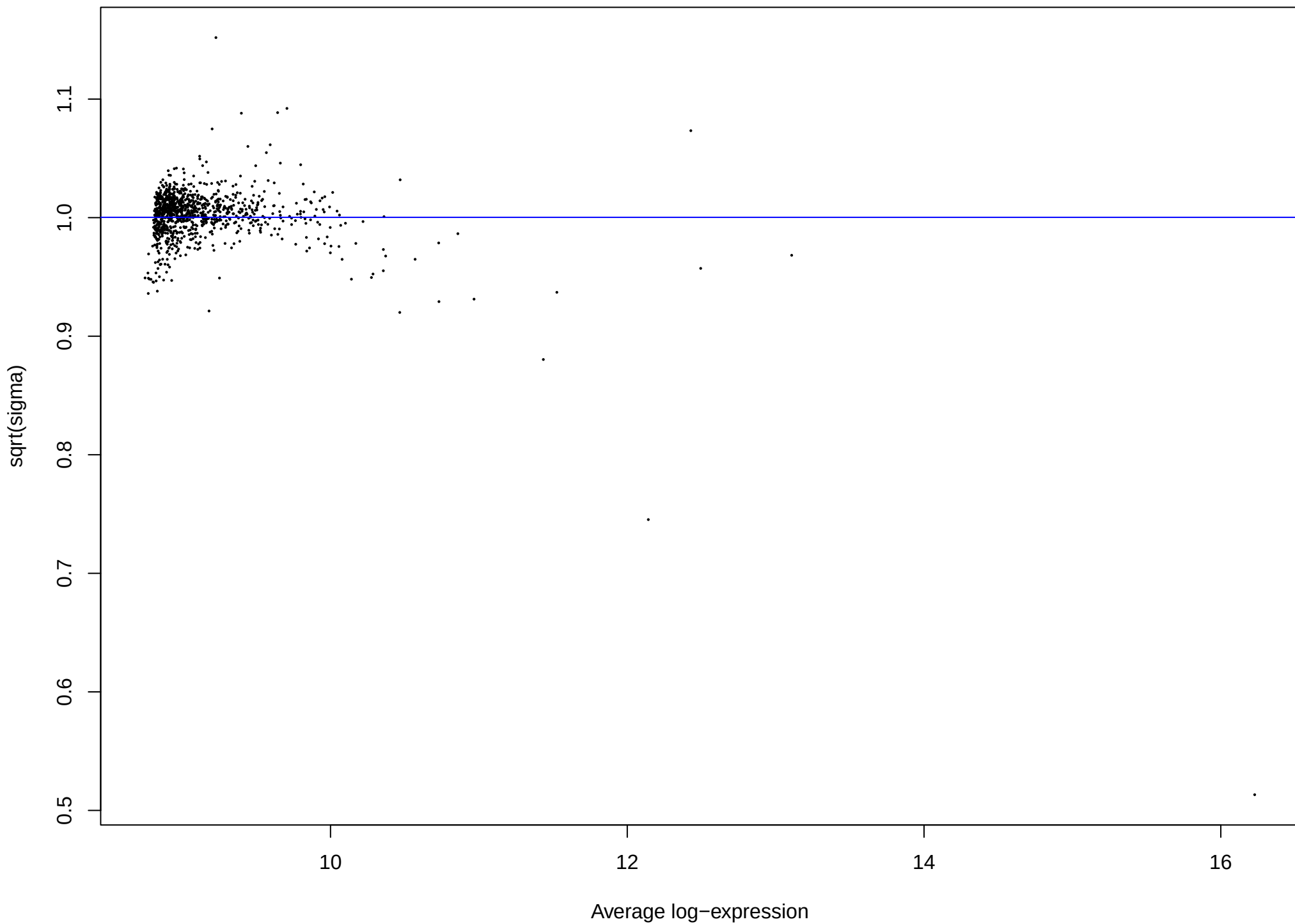
Final model Non-neuronal: Mean-variance trend
