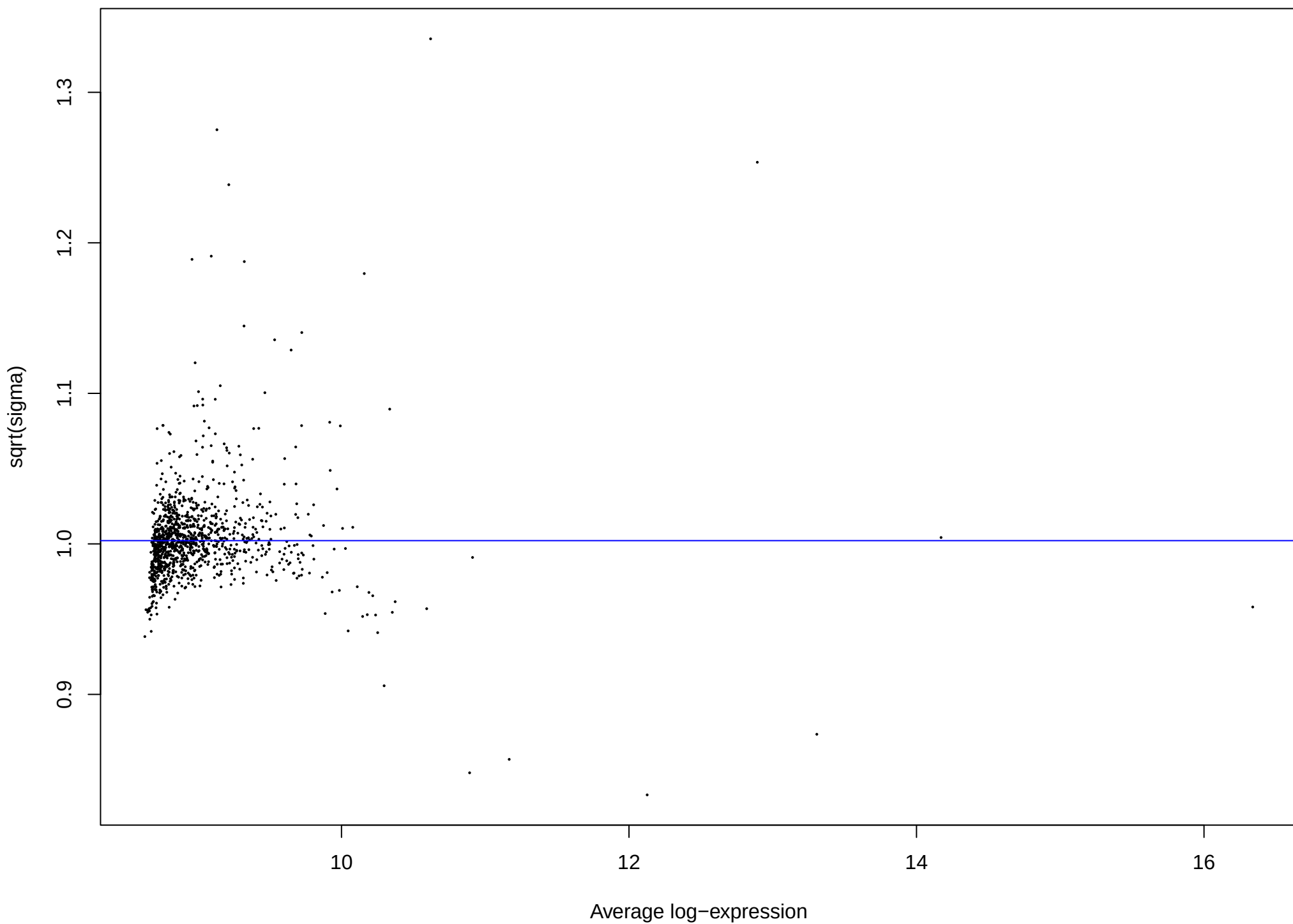
Final model Vip: Mean–variance trend
