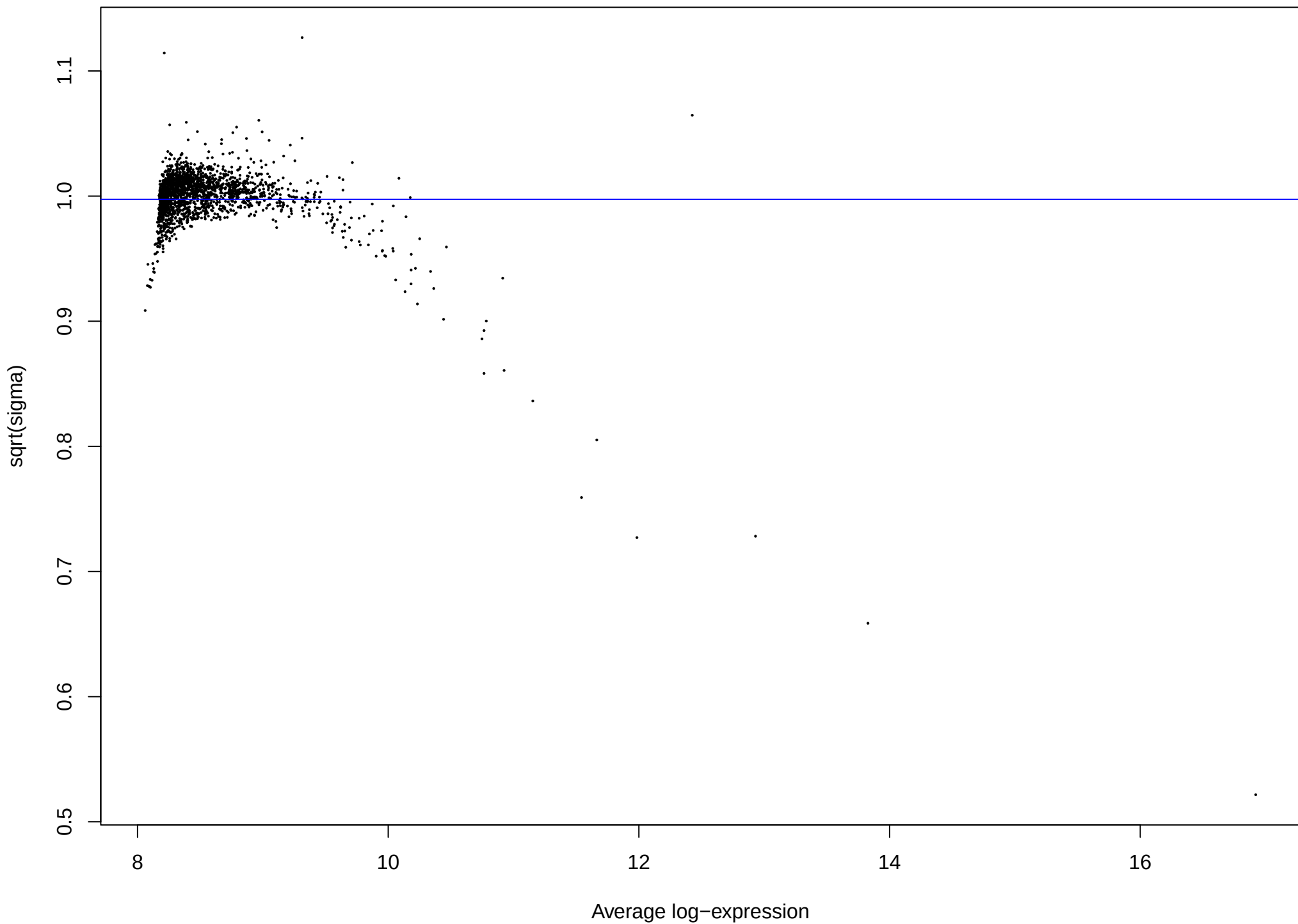
Final model L2_3_IT: Mean-variance trend
