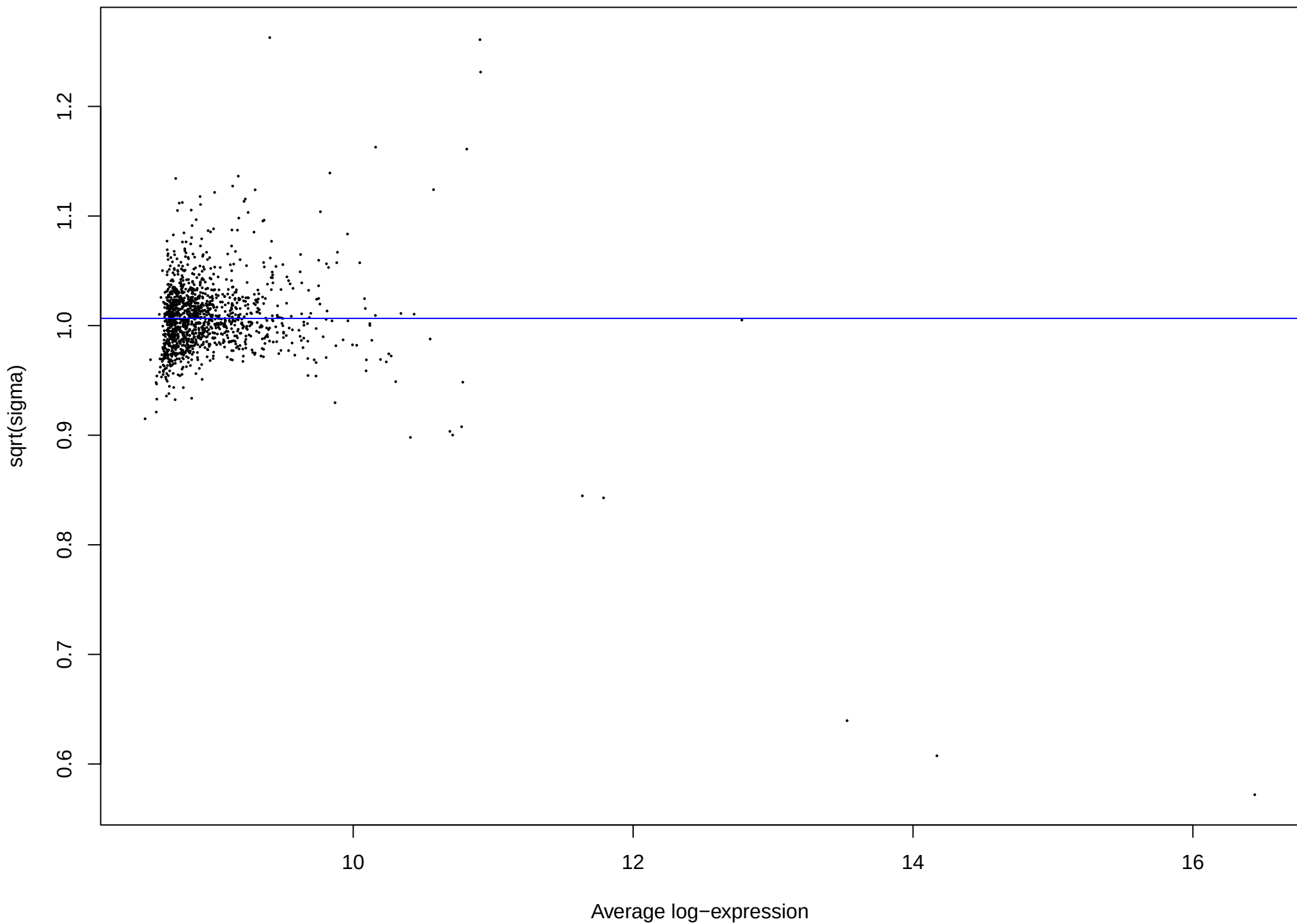
Final model Sncg: Mean-variance trend
