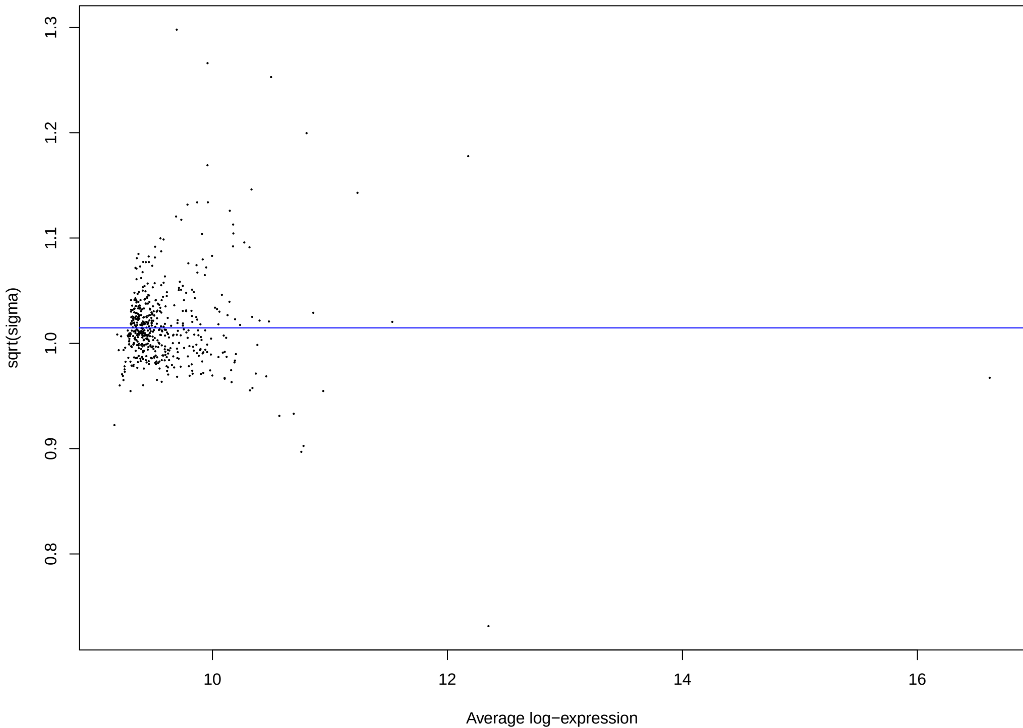
Final model Oligo: Mean–variance trend
