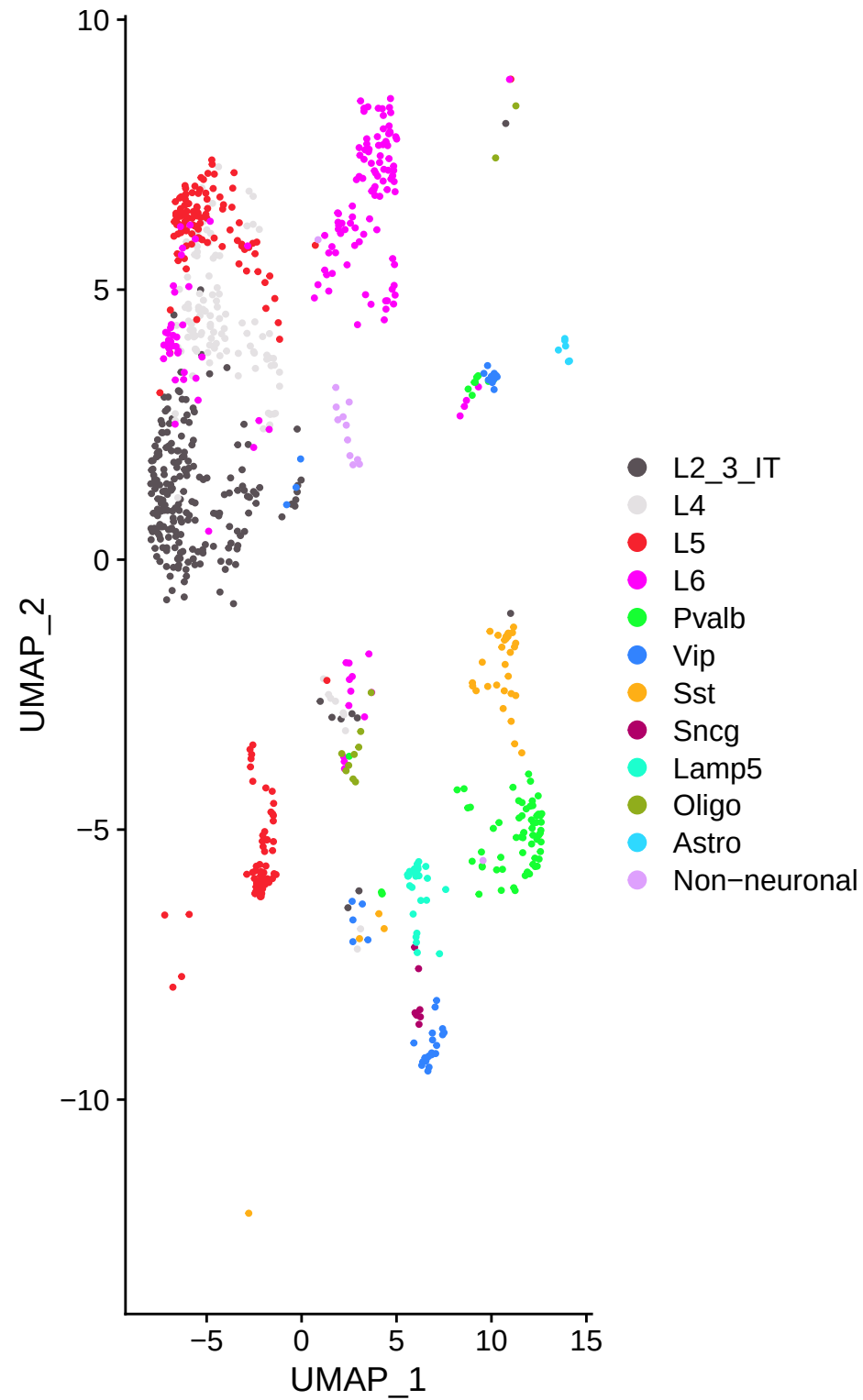
MUT_Mecp2
