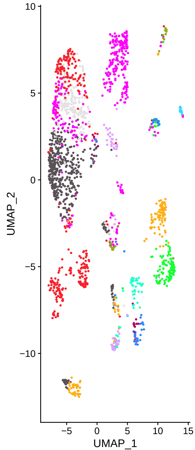
WT_Mecp2
