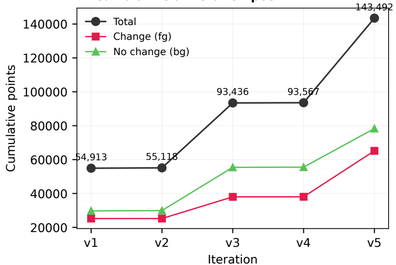
B. Cumulative annotation pool
