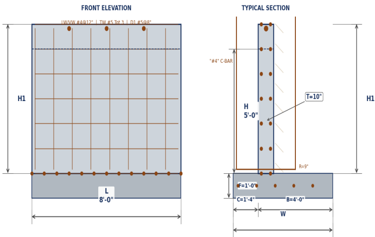
STRAIGHT HEADWALL (D89A)
