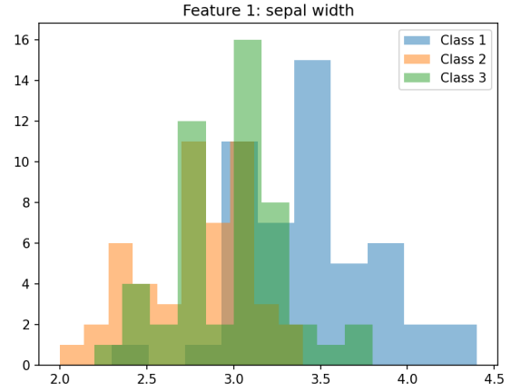
(b) Sepal width and the overlap between the three classes
