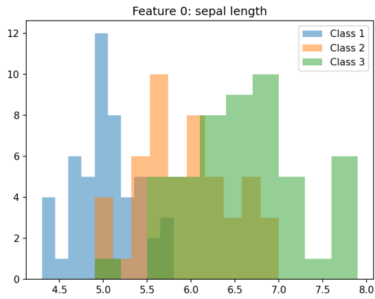
(a) Sepal length and the overlap between the three classes
