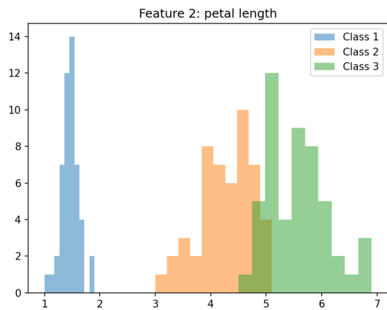
(c) Petal length and the overlap between the three classes
