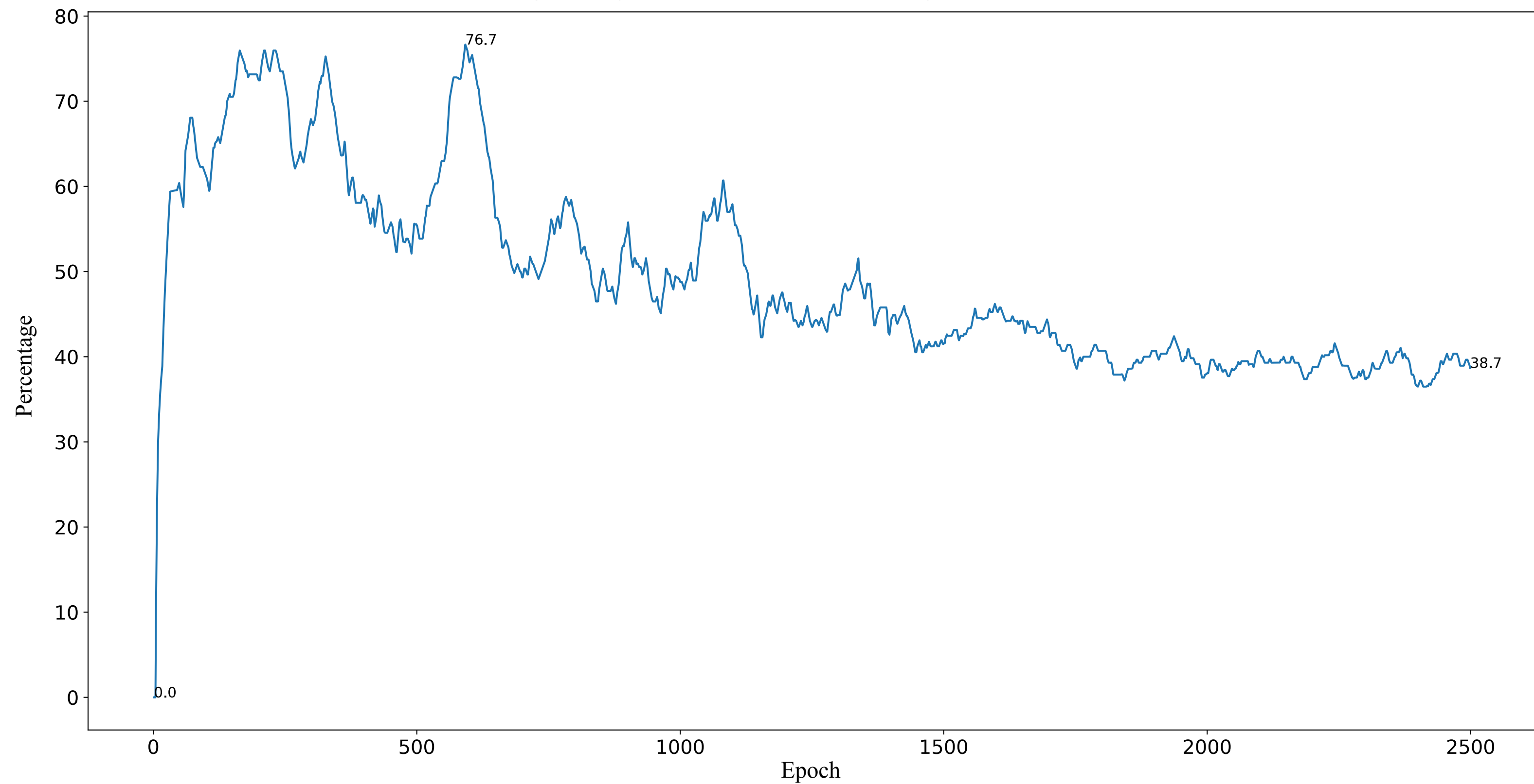
Moving average of Minimum Dominating Set relative size
