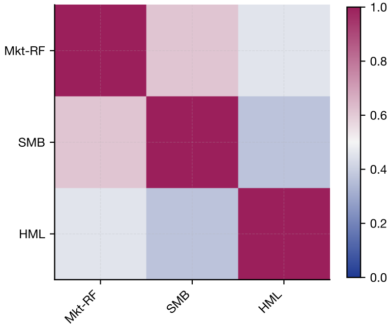
\chi matrix
