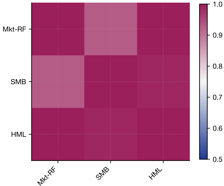
\eta matrix
