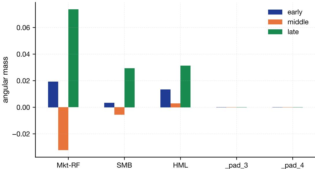
Rolling empirical spectral measure
