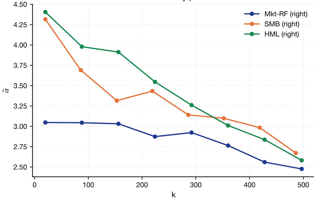
Hill stability plot
