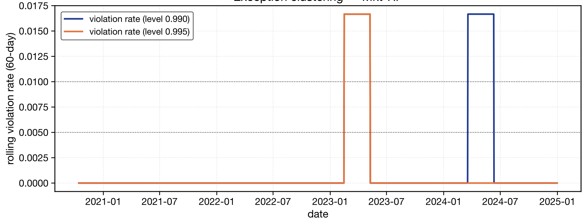
Exception clustering — Mkt-RF
