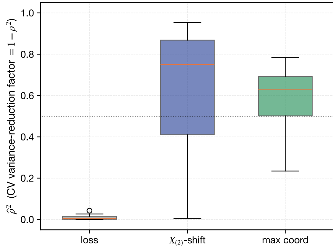
Surrogate kind drives correlation
