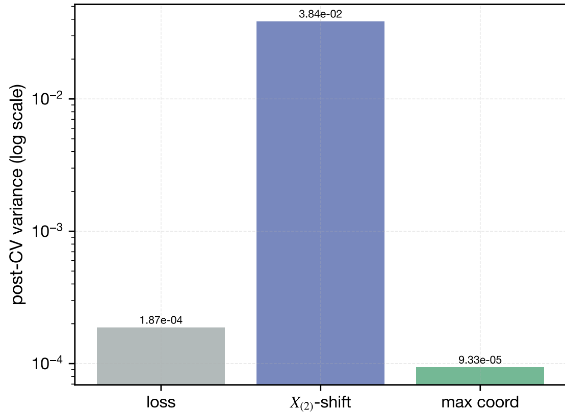
Post-CV variance: lower is better
