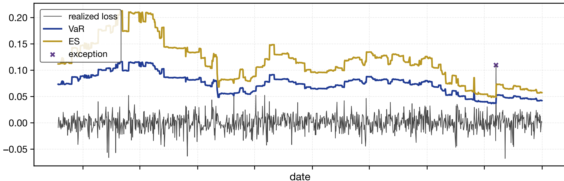
VaR / ES at confidence level 0.995
