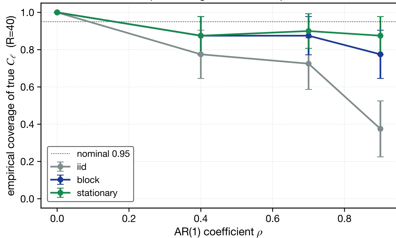
Bootstrap coverage vs serial dependence
