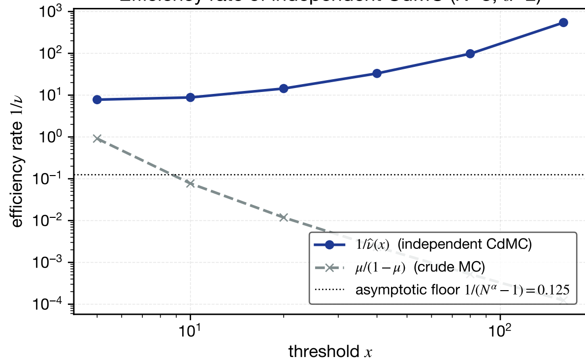
Efficiency rate of independent CdMC ( N=3 , \alpha=2 )
