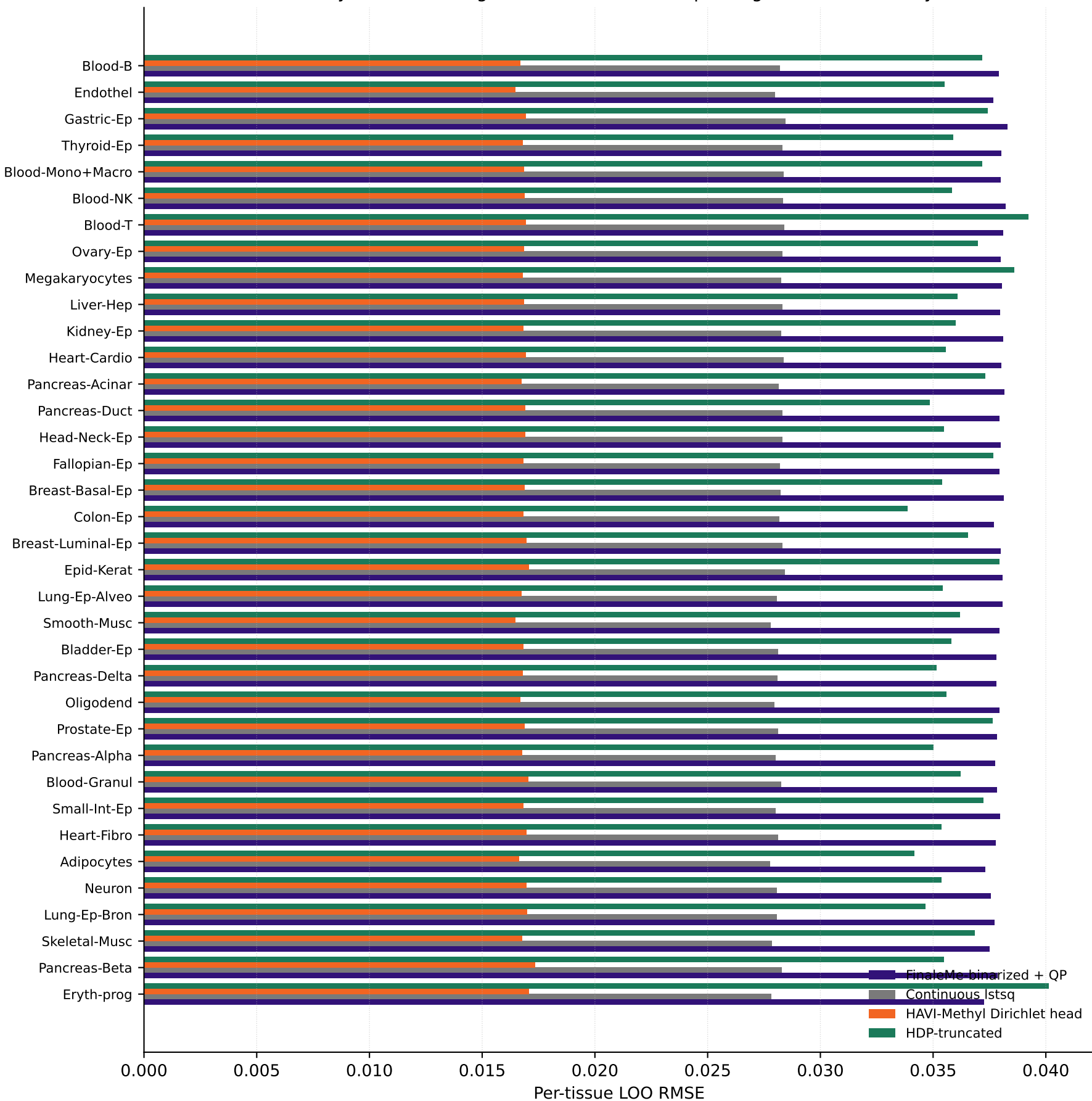
Per-tissue leave-one-out RMSE on real Loyfer U25 panel (36 cell types x 900 markers) Sorted by HAVI advantage over continuous ltsq; orange shortest at every row.
