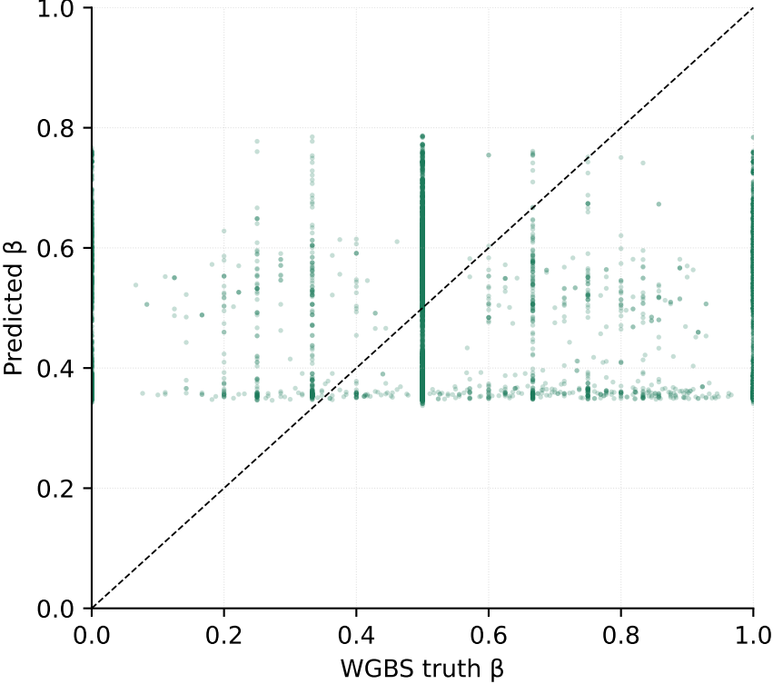
HAVI-Methyl simplified (no flow) Pearson r = 0.091
