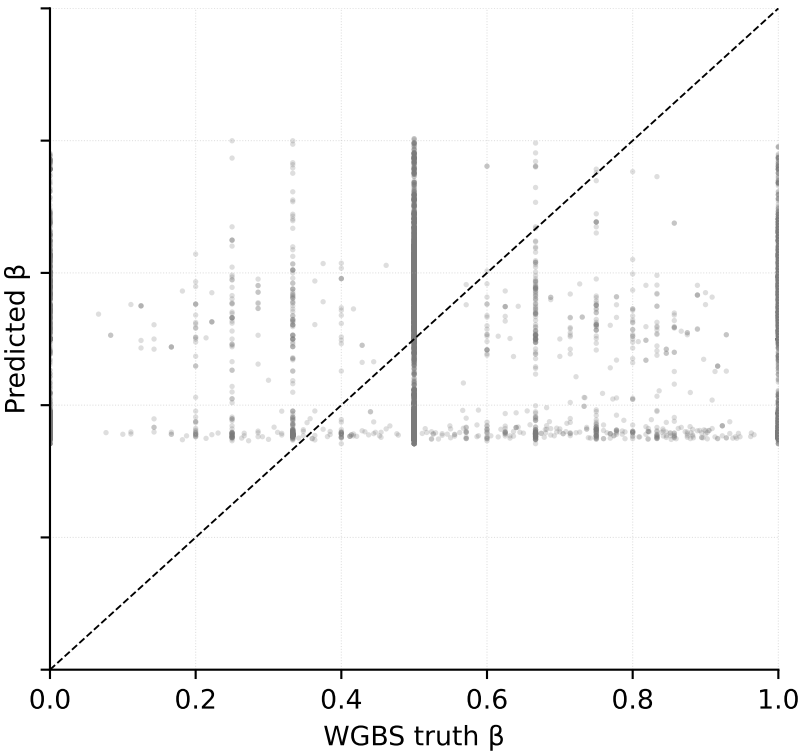
HAVI-Methyl simplified (no hierarchy) Pearson r = 0.088
