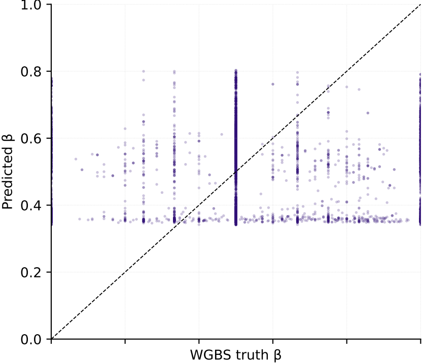
FinaleMe-style HMM Pearson r = 0.088
