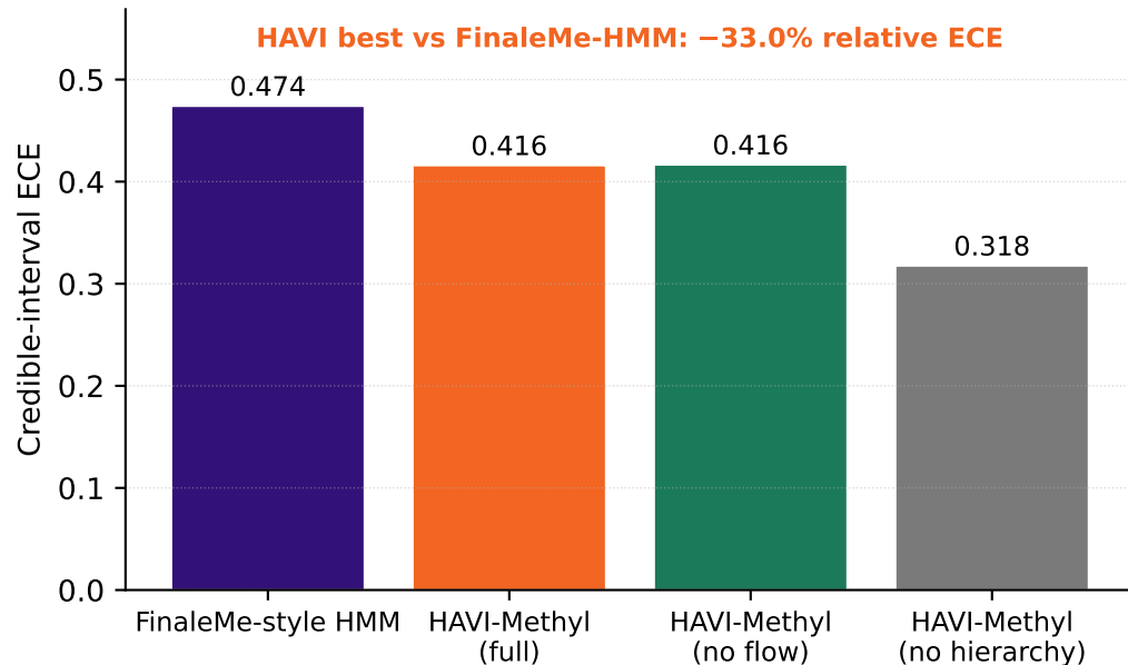
Calibration (lower is better)
