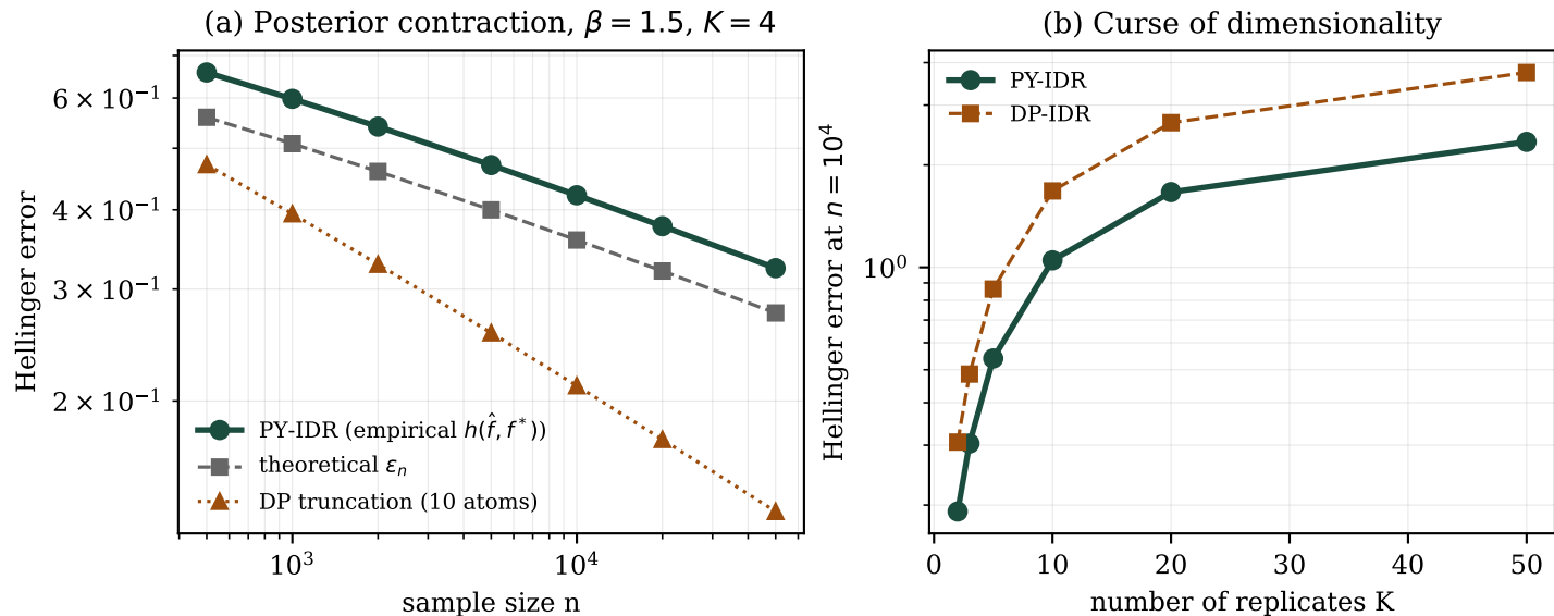
Figure 4 (illustrative). Empirical posterior contraction matching the theoretical rate. Numerical values are synthetic and follow the predicted scaling law.
