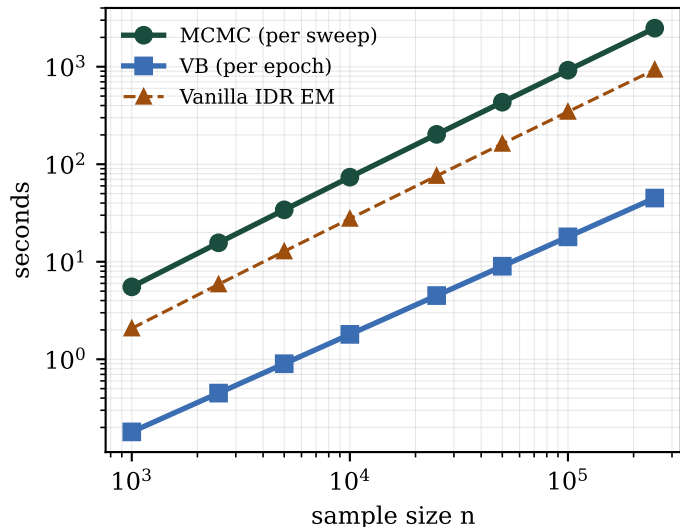
(a) Per-iteration cost
