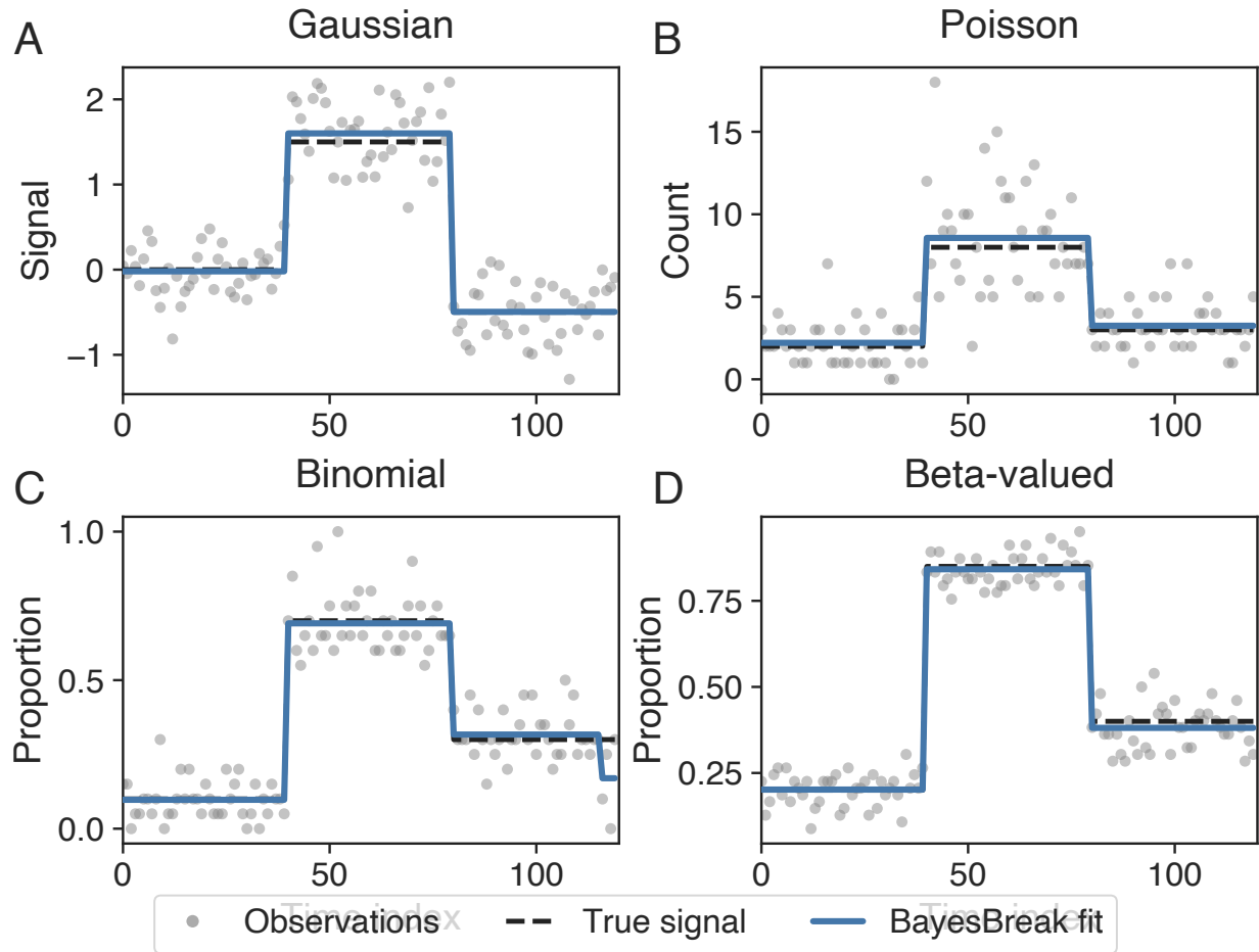
Figure 10. Executed family showcase. Gaussian, Poisson, and Binomial use closed-form local conjugate integration; the Beta-valued response uses deterministic one-dimensional quadrature.
