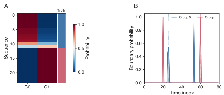
(b) Latent-group assignments and group-specific boundary marginals.
