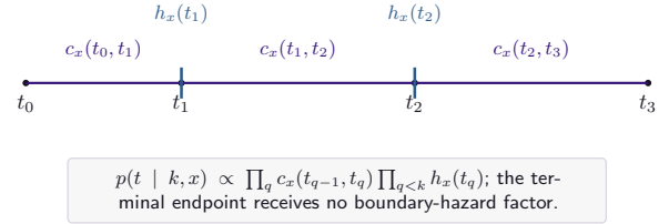
Figure 3. Design-dependent partition prior. Segment cohesion and interior-boundary hazard represent different prior assumptions. The terminal endpoint receives no boundary-hazard factor.
