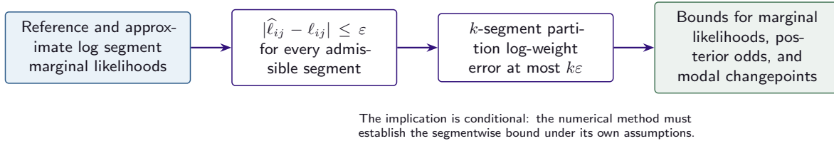
Figure 6. Propagation of a uniform log marginal-likelihood error through the partition recursions. The global bounds require an independently established segmentwise error bound; they do not provide such a bound for a numerical approximation.
