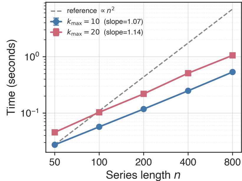
Runtime vs. series length
