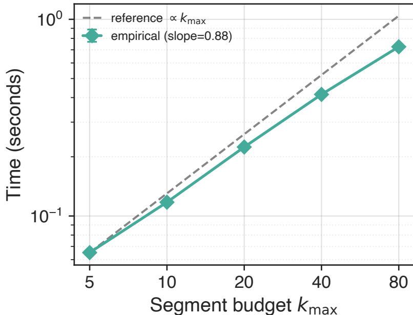
Runtime vs. k_{\max} ( n = 200 )
